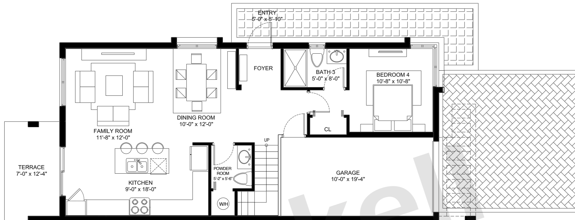
FIRST FLOOR
