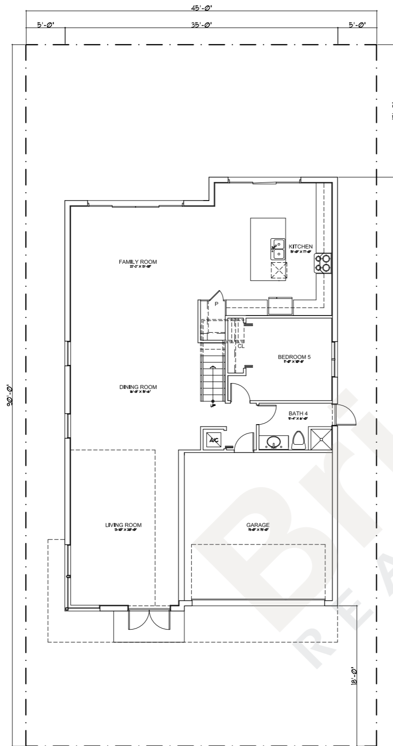
1 st Floor
