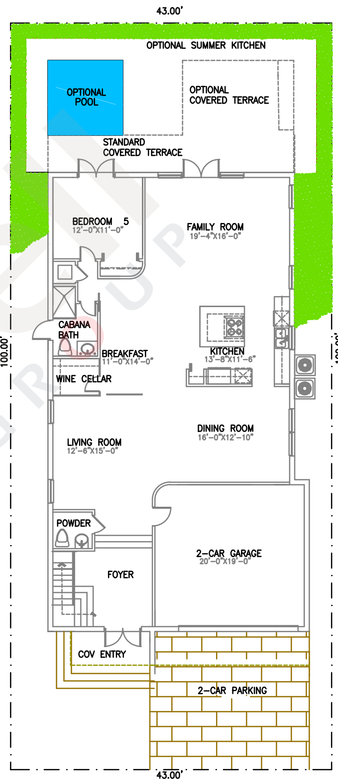
First Floor
